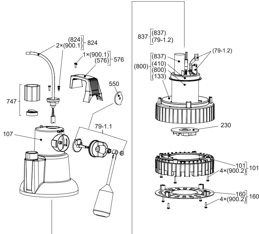
Fig. 5: Exploded view
