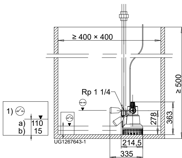
Fig. 3: Dimensions of AmaDrainer 302/303
