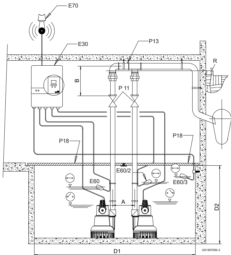
Fig. 4: Installation example of a dual-pump station
