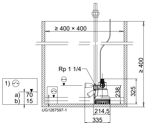
Fig. 2: Dimensions of AmaDrainer 301
